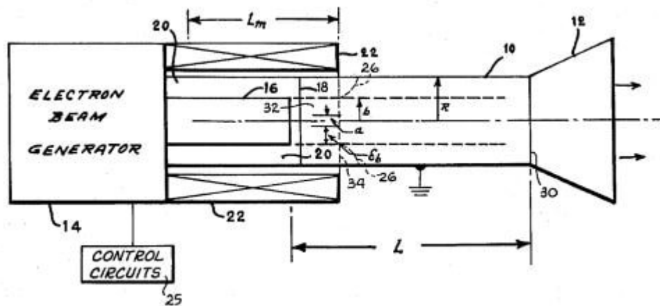
Figure 8. Vircator microwave weapon is mounted on a satellite, and emits a beam that is about 1/2 inch in diameter. The beam travels at the speed of light, and is invisible, just like the microwaves in your oven.
