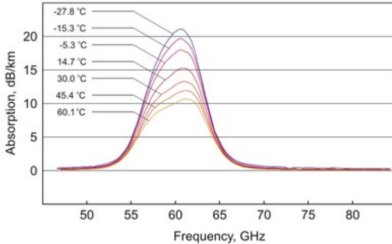
Fig. 2. Absorption profiles in air at several temperatures.
